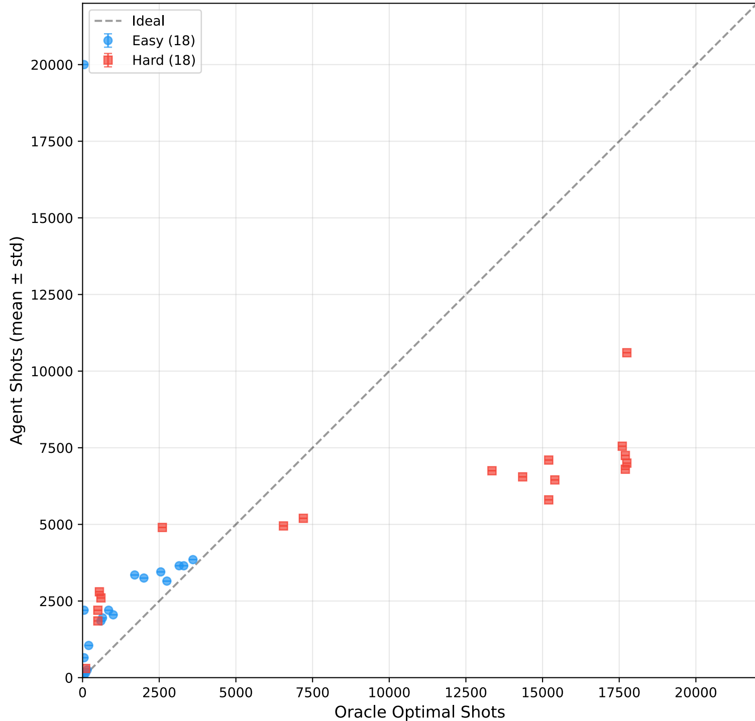
Multi-Run Eval (1 runs) — GENERIC
