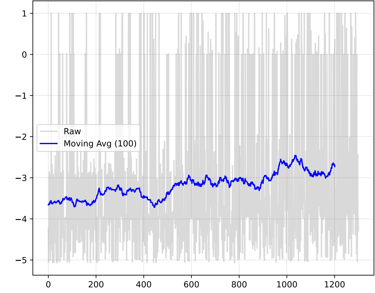
Training Rewards
