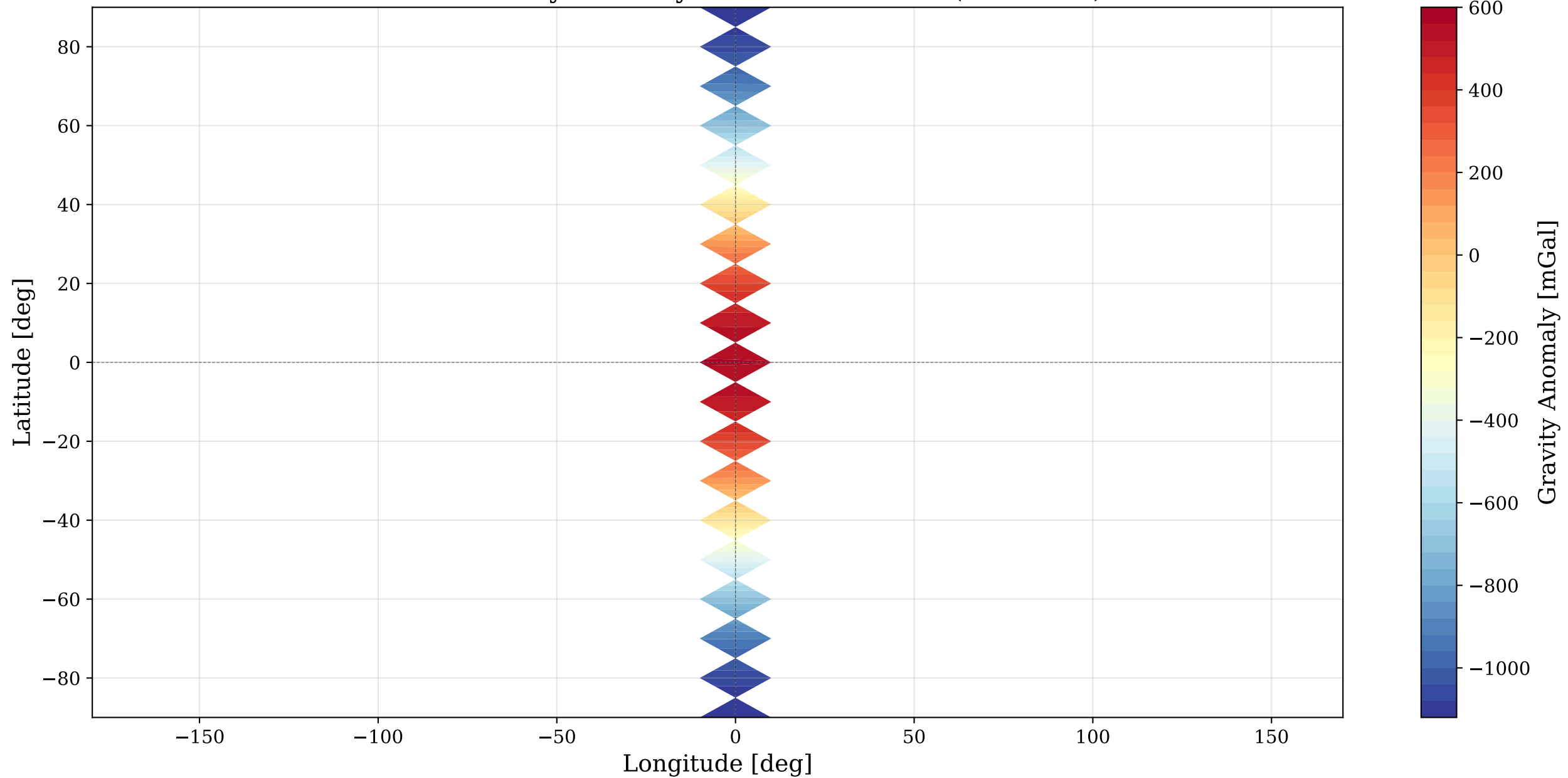
GGM05C Gravity Anomaly at 400km Altitude (nmax=70)
