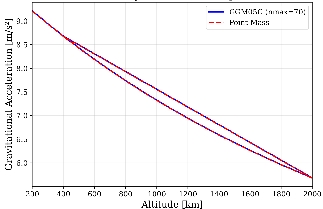
(a) Gravity vs Altitude at Equator
