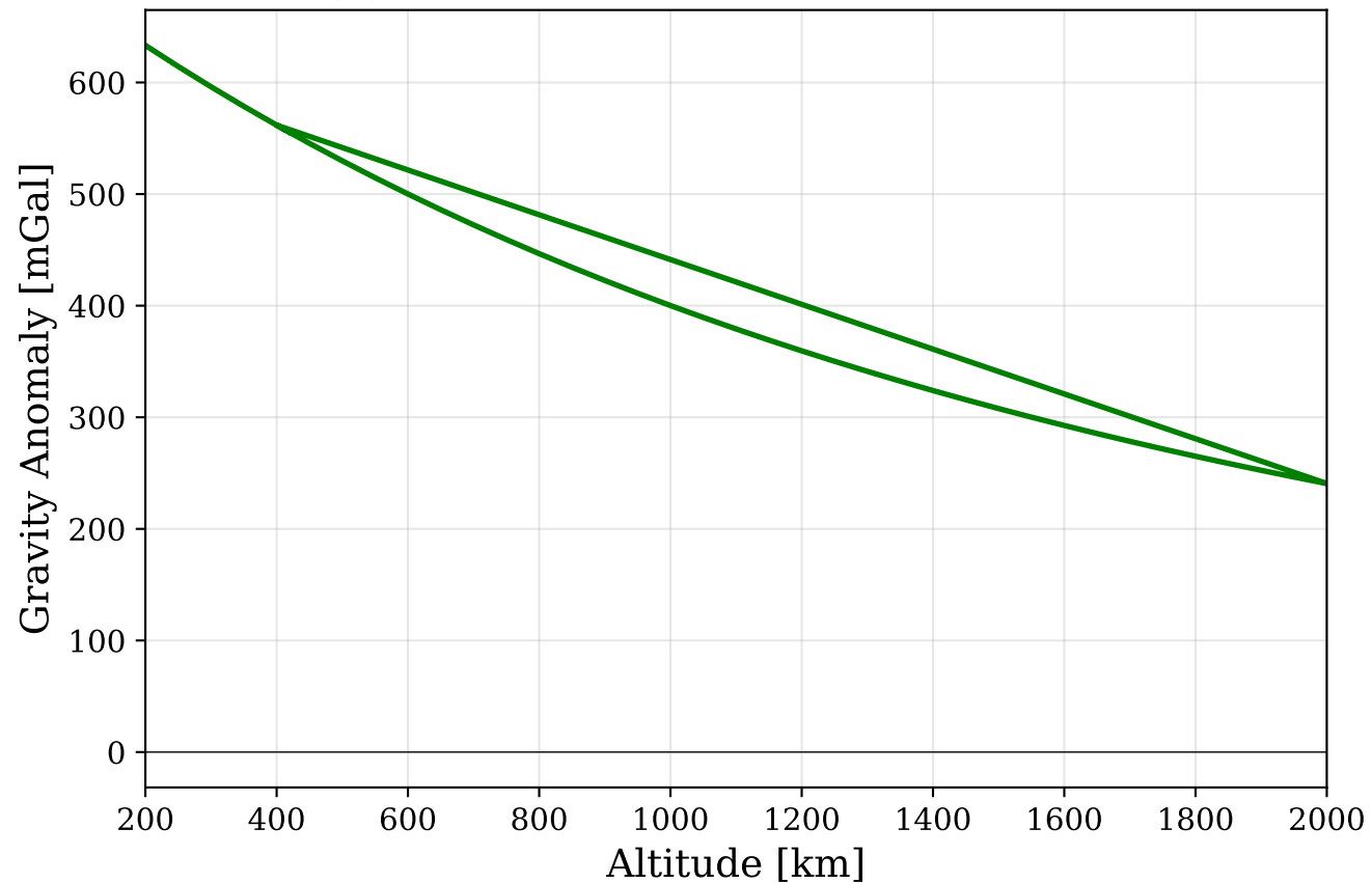
(b) GGM05C - Point Mass Difference
