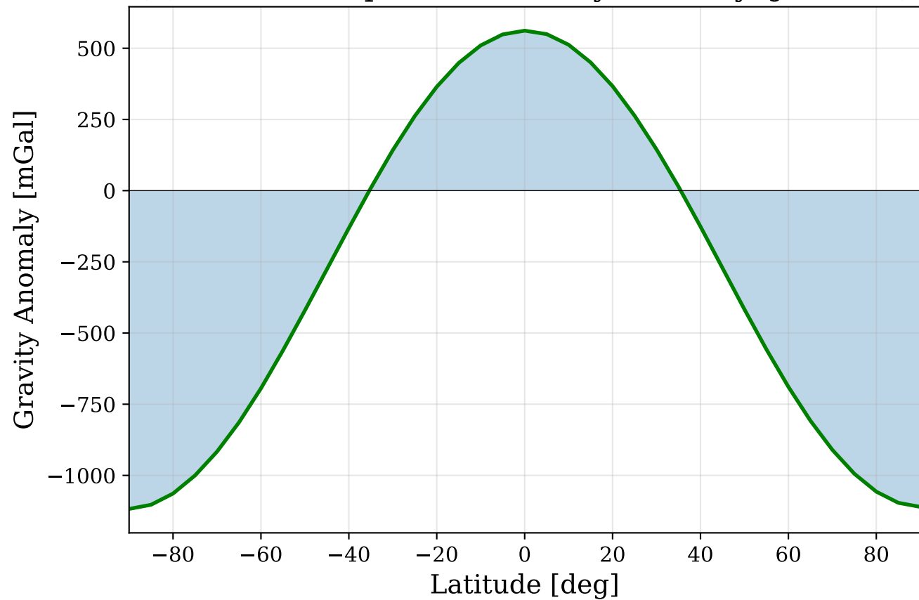
(b) Latitude-dependent Gravity Anomaly (J2 effect)
