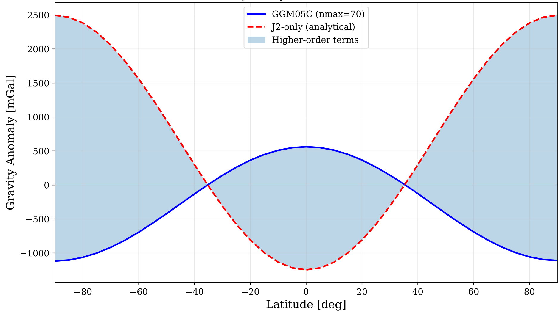
GGM05C vs J2-only Model at 400km Altitude
