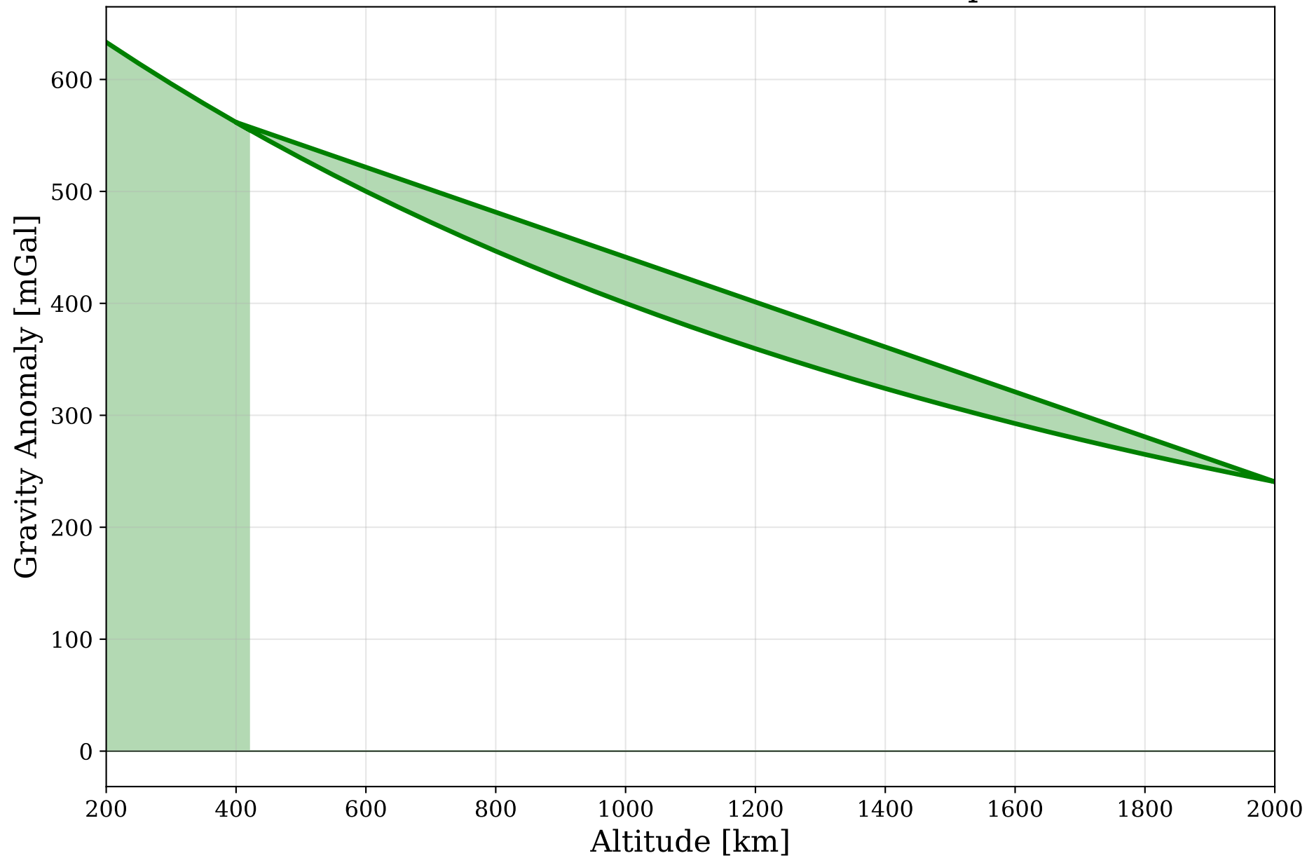
GGM05C - Point Mass Difference at Equator
