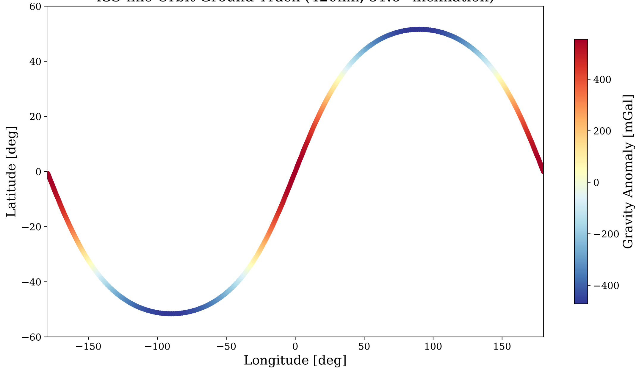
ISS-like Orbit Ground Track (420km, 51.6° inclination)
