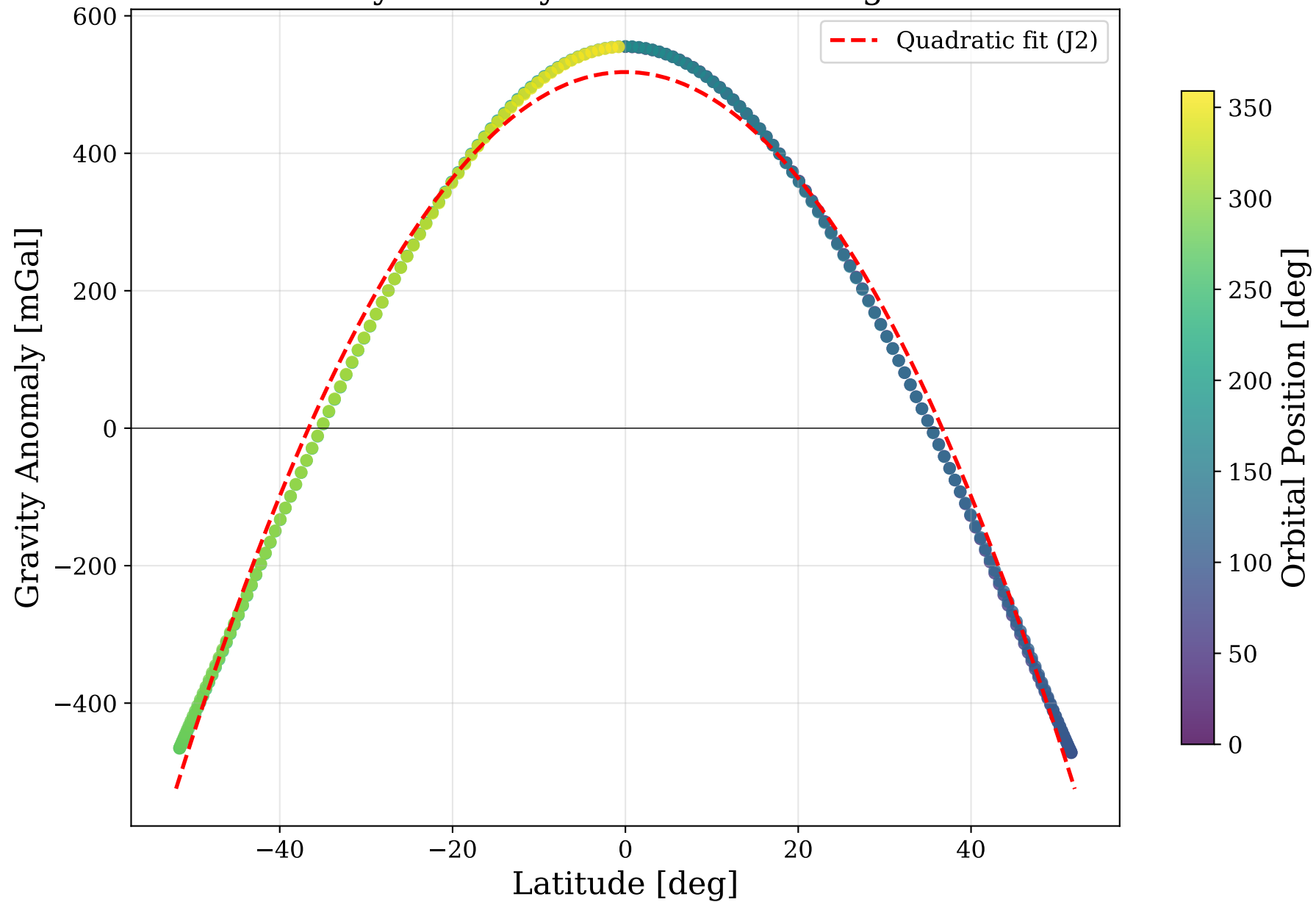
Gravity Anomaly vs Latitude Along Orbit
