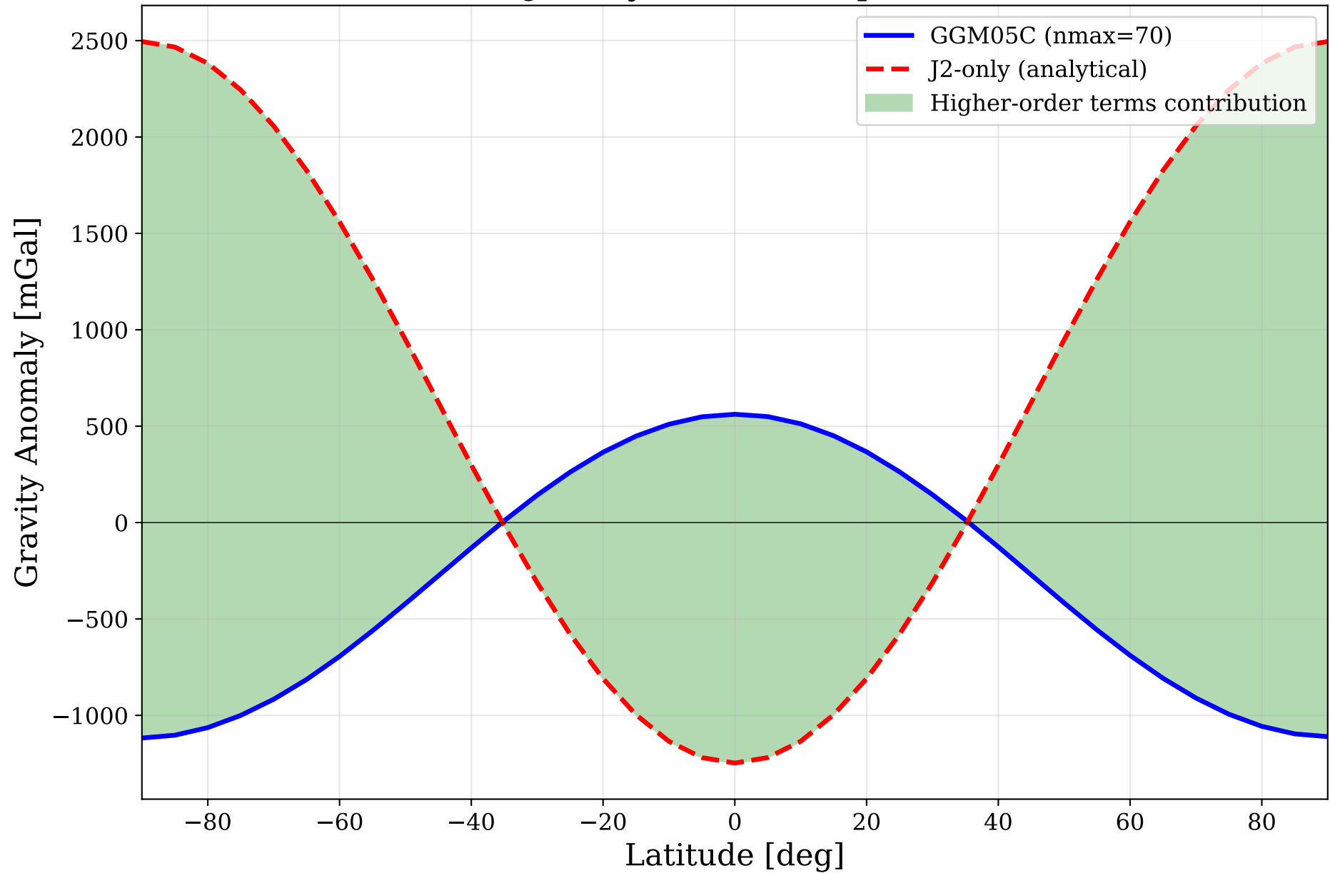
GGM05C vs J2-only Model Comparison at 400km
