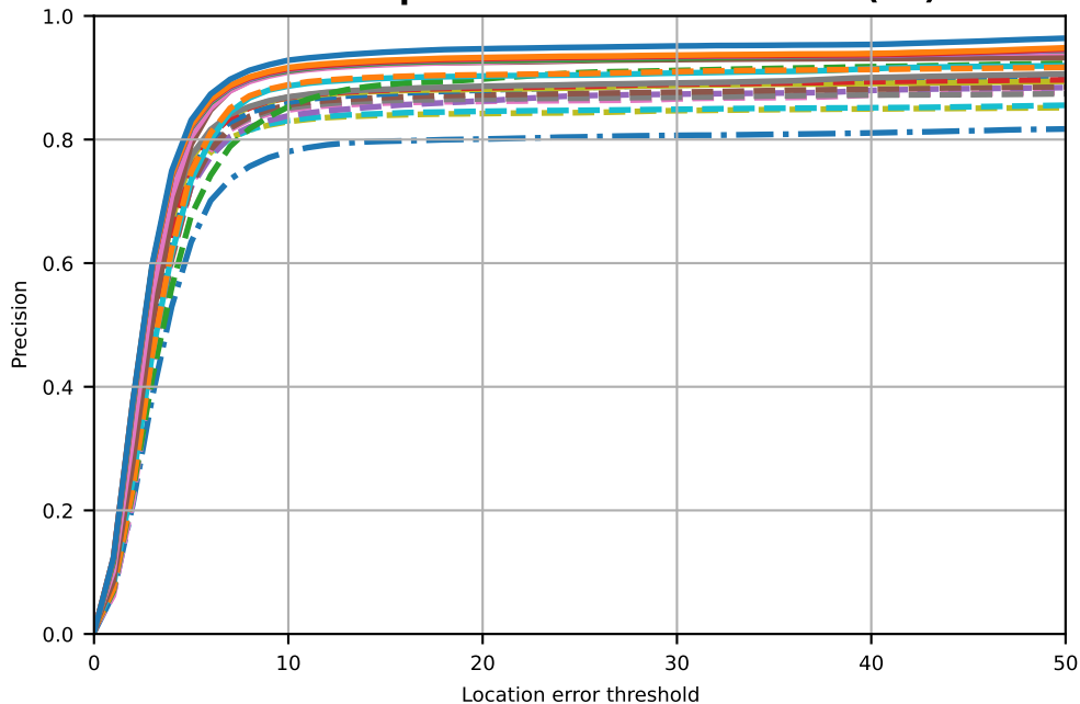
Precision plots of OPE - Normal Size(32)
