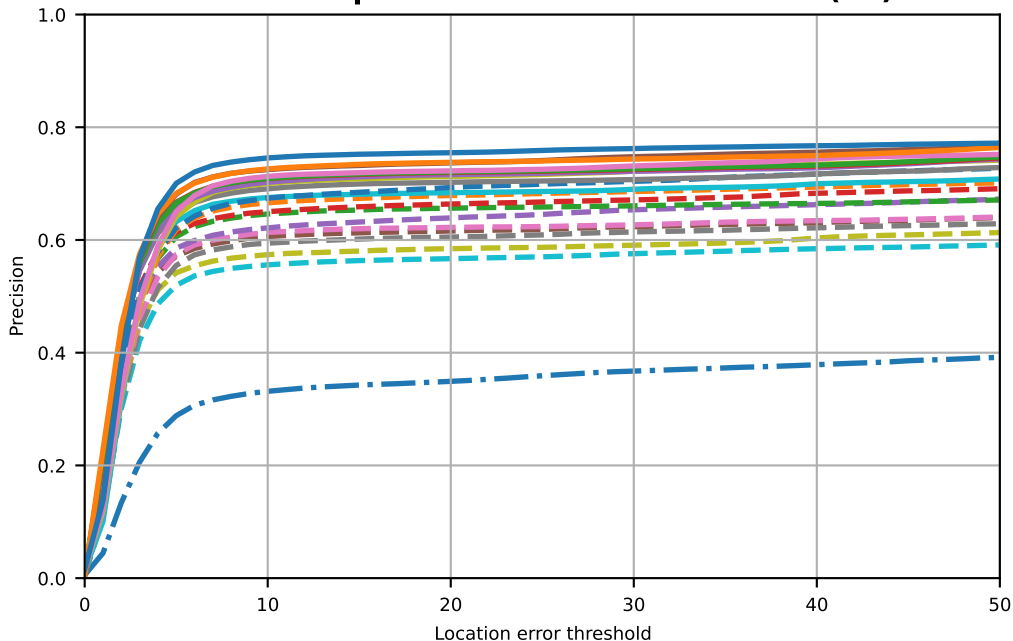
Precision plots of OPE - Scale Variation(27)
