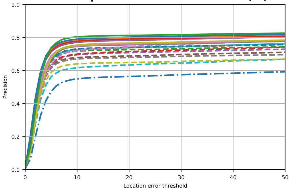
Precision plots of OPE - Thermal Crossover(81)
