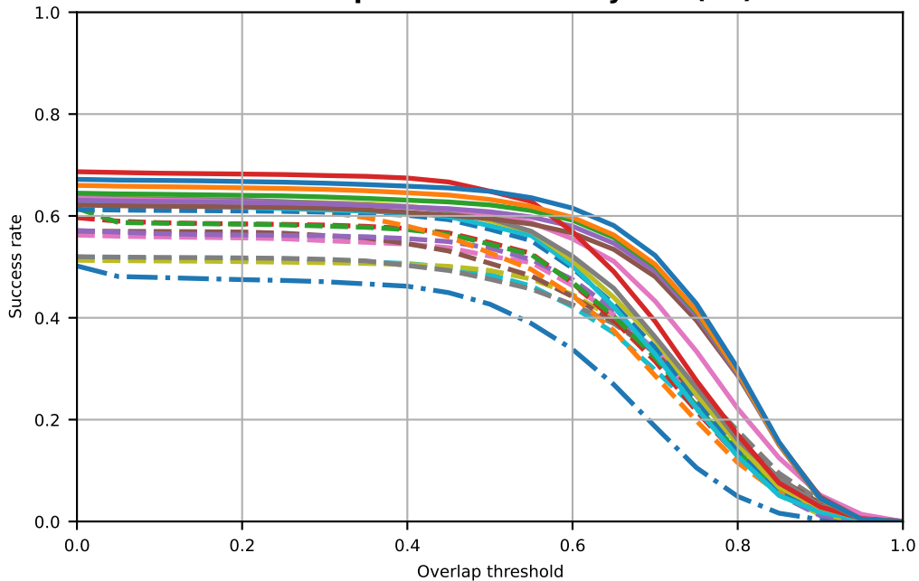
Success plots of OPE - Tiny Size(33)
