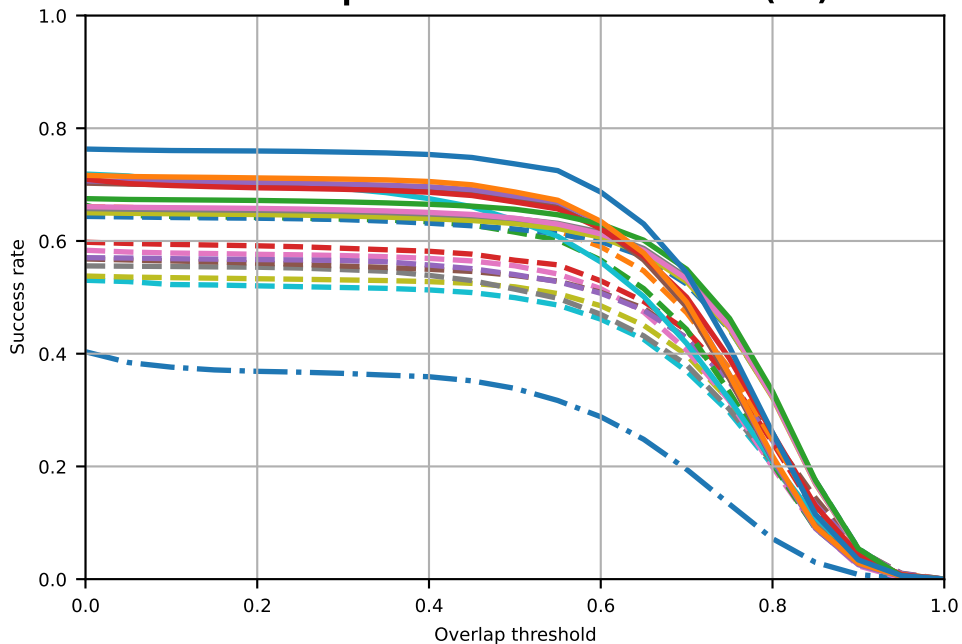
Success plots of OPE - Fast Motion(52)
