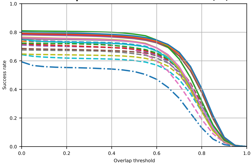
Success plots of OPE - Thermal Crossover(81)
