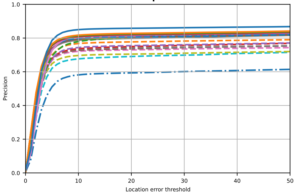
Precision plots of OPE
