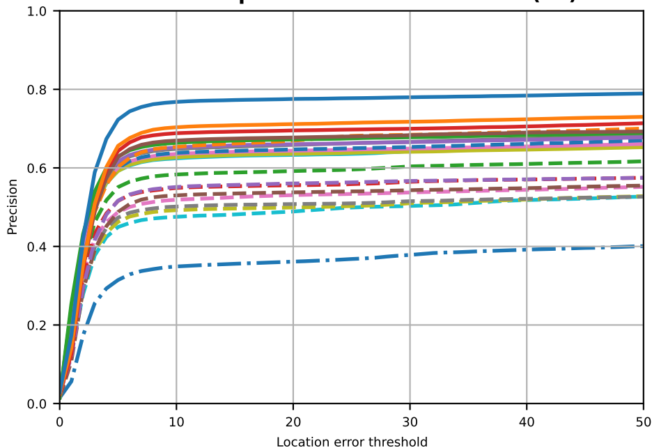
Precision plots of OPE - Out-of-View(31)
