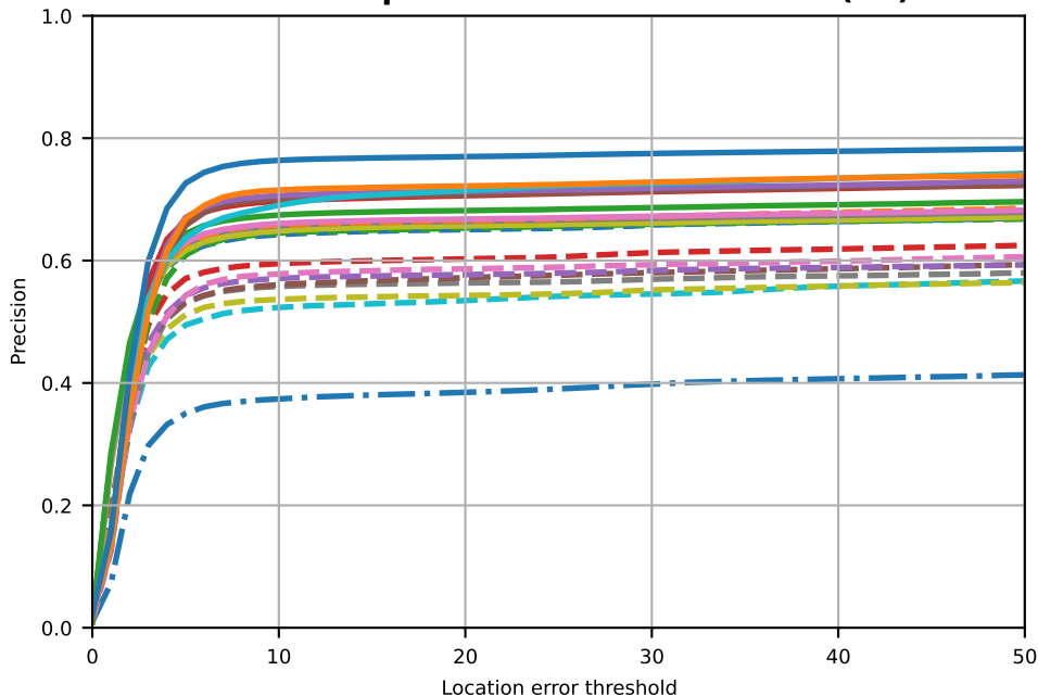
Precision plots of OPE - Fast Motion(52)
