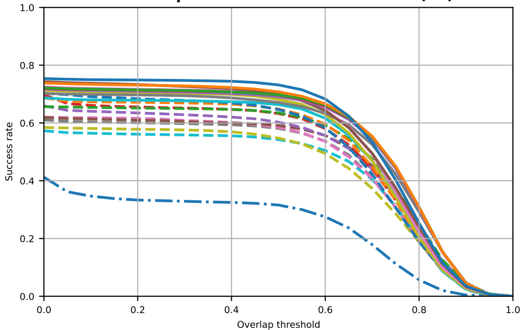
Success plots of OPE - Scale Variation(27)
