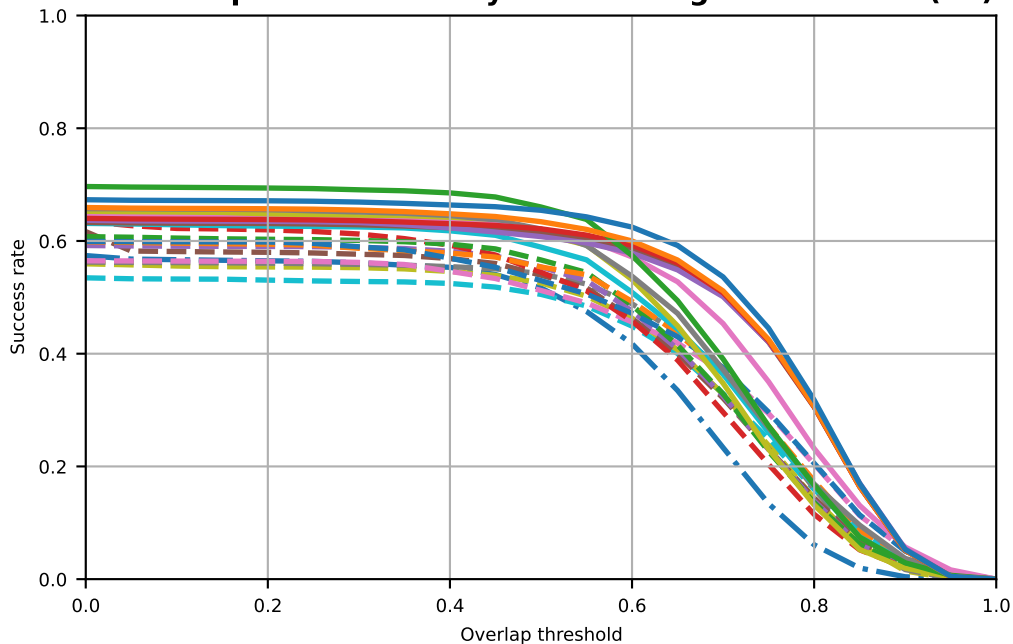
Success plots of OPE - Dynamic Background Clutter(21)
