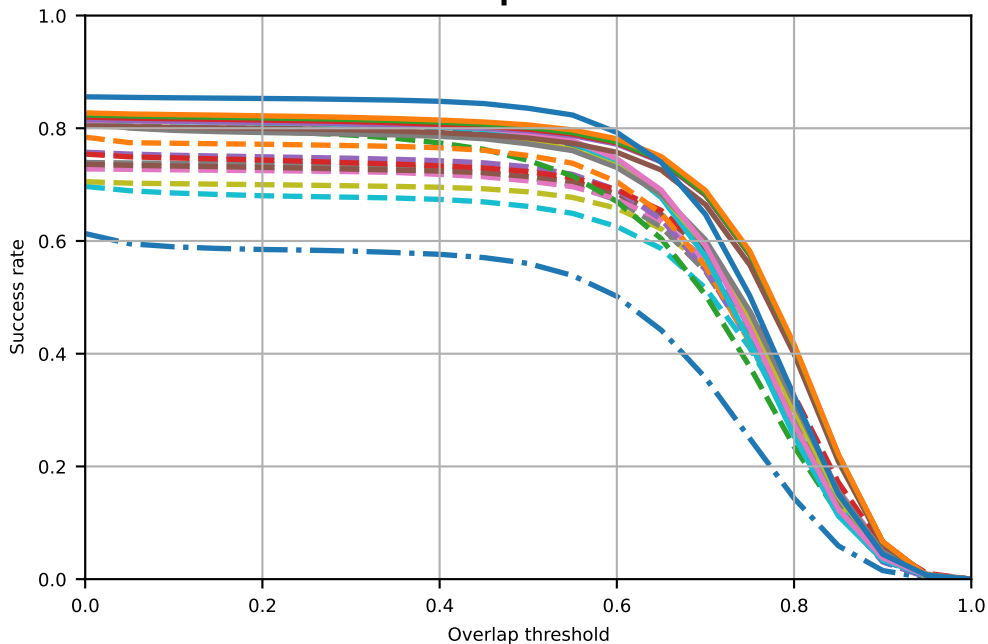
Success plots of OPE
