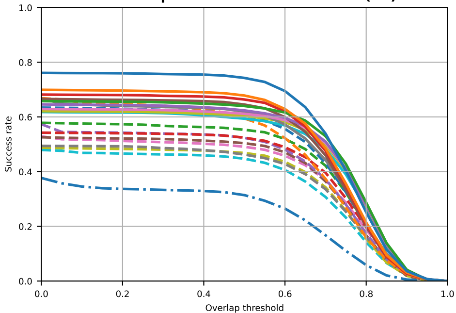
Success plots of OPE - Out-of-View(31)
