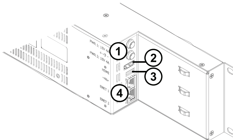
Figure 4 Ultritouch-2-HR — Rear Panel, Side View
