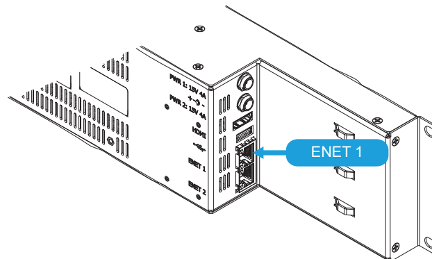
Figure 9 Ultritouch-2-HR — ENET 1 Connection
