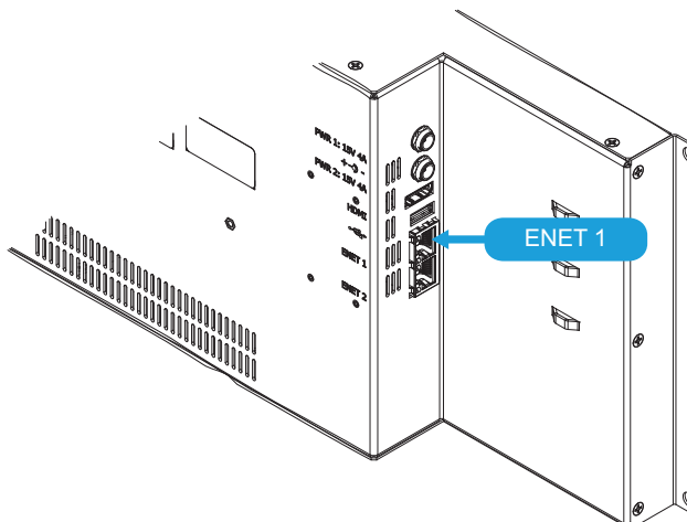
Figure 10 Ultritouch-4 — ENET 1 Connection
