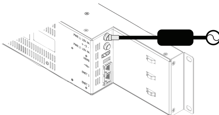
Figure 11 Ultritouch-2-HR — Primary Power Connection
