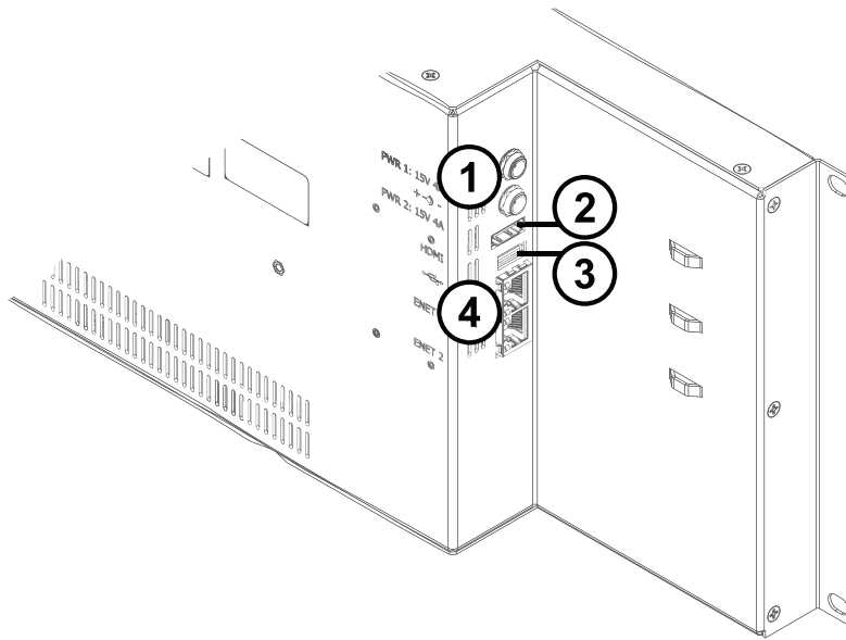
Figure 5 Ultritouch-4 — Rear Panel, Side View
