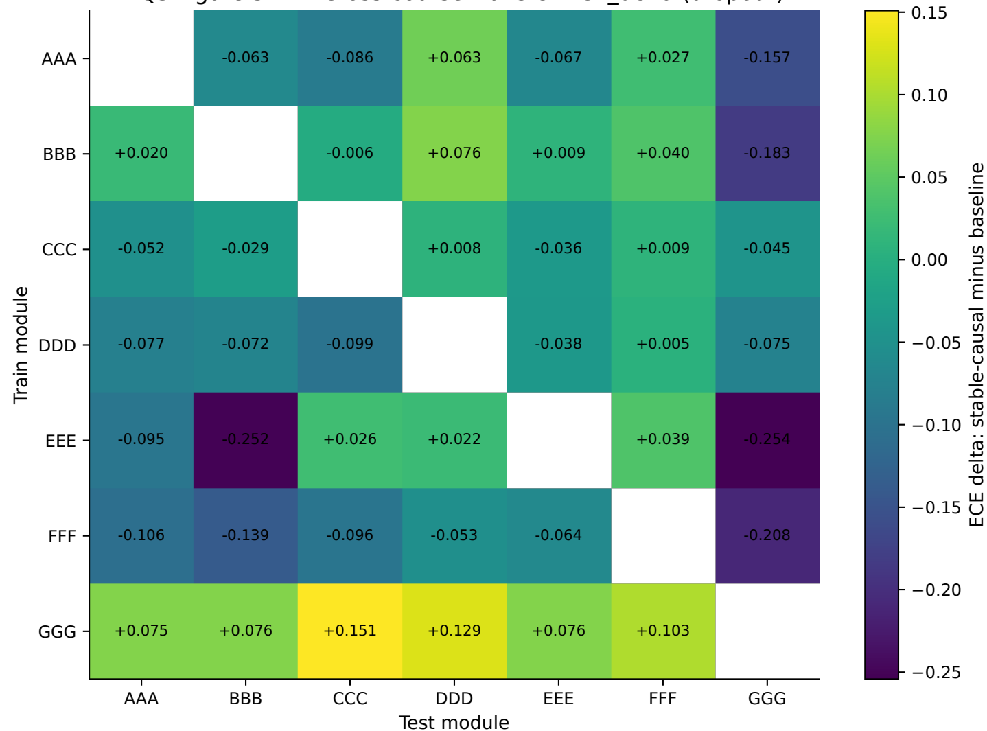
RQ3 Figure 3.1 — Cross-course transfer ECE_delta (dropout)
