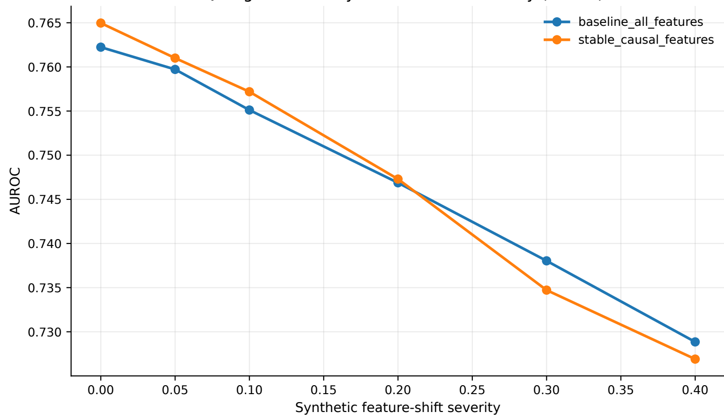
RQ3 Figure 3.2 — Synthetic shift sensitivity (failure)
