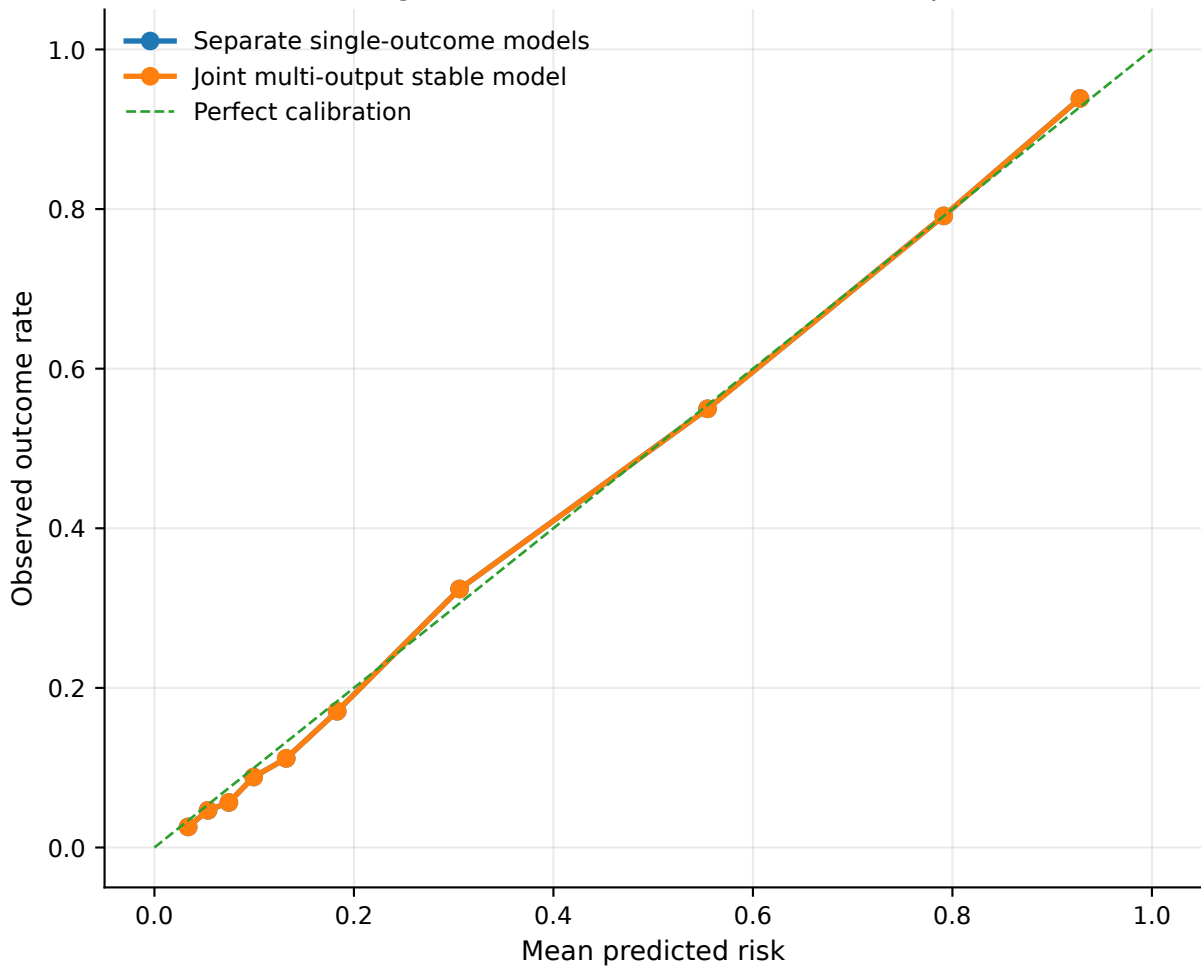
RQ6 Figure 6.2 — Calibration curve (dropout)
