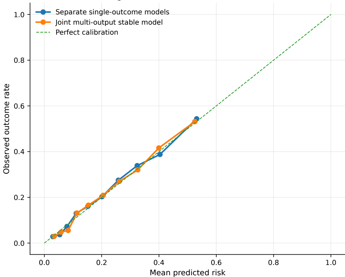
RQ6 Figure 6.2 — Calibration curve (failure)
