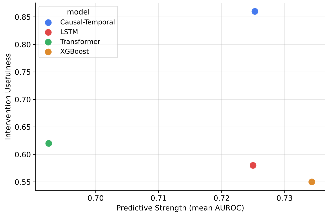
Figure 1.2 Accuracy-actionability trade-off
