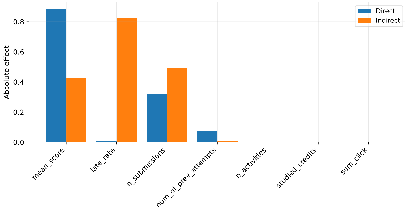
Figure 2.2 — Direct and mediated pathway decomposition
