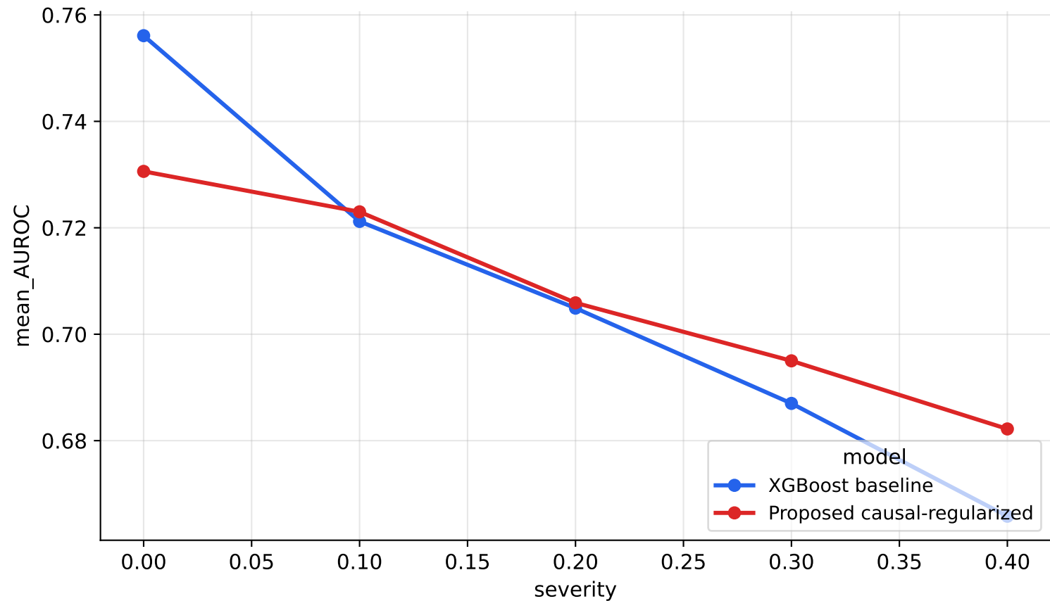
Figure 3.2 Performance decay under synthetic shift severity
