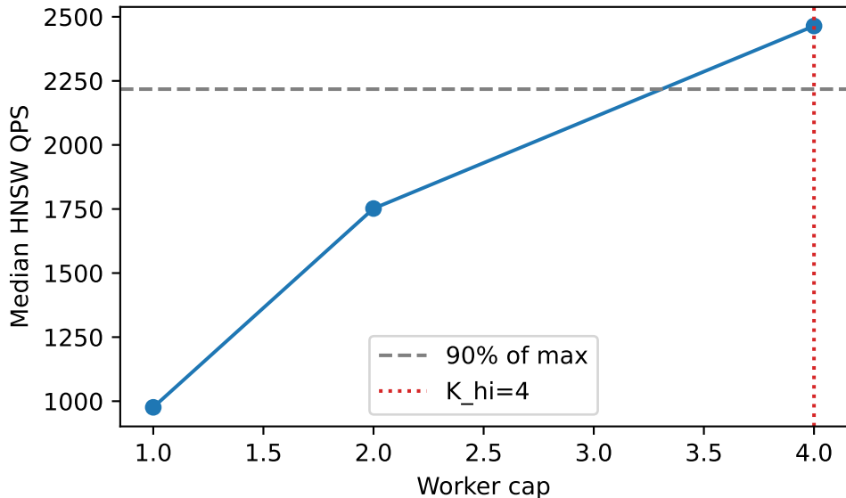
Apple M4 CPU-only HNSW scaling
