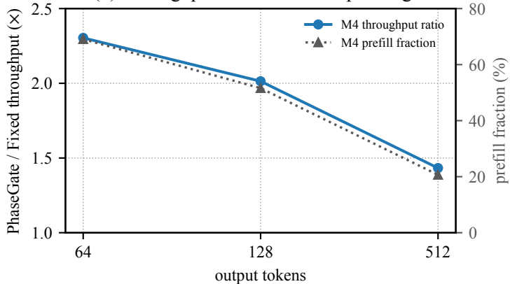
(b) Throughput ratio versus output length
