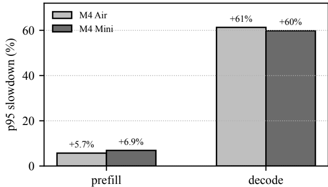
(a) HNSW phase asymmetry on two M4 devices
