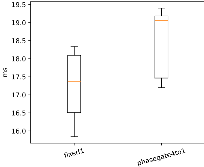
p95 transition gap
