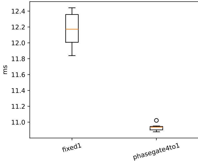
p99 inter-token gap
