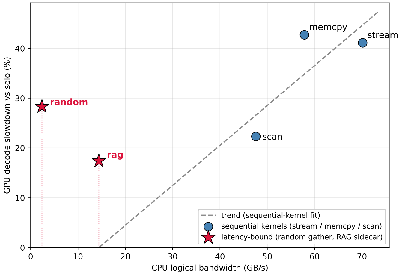
Decode slowdown vs CPU logical bandwidth (M4, 1.5B)
