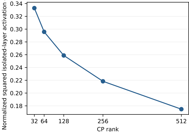
Isolated classifier.0 activation distortion
