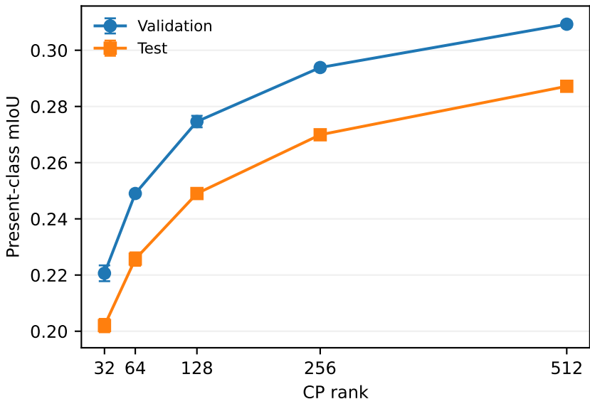
Zero-shot segmentation after CP replacement
