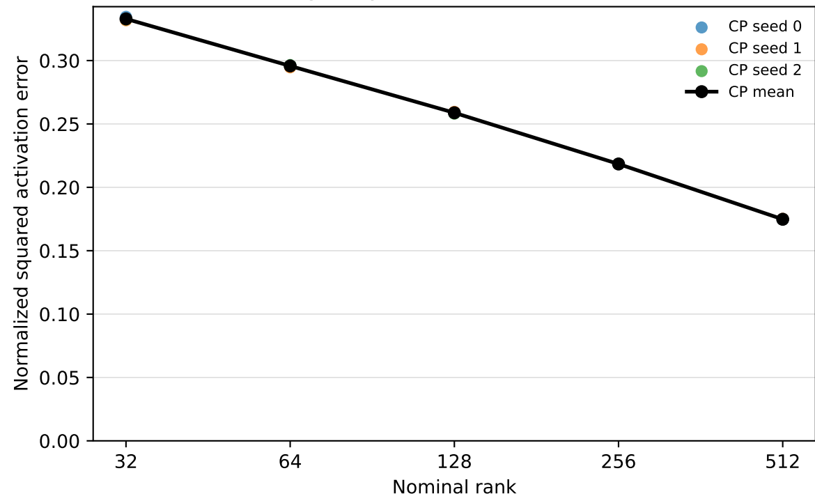
Target-layer activation distortion
