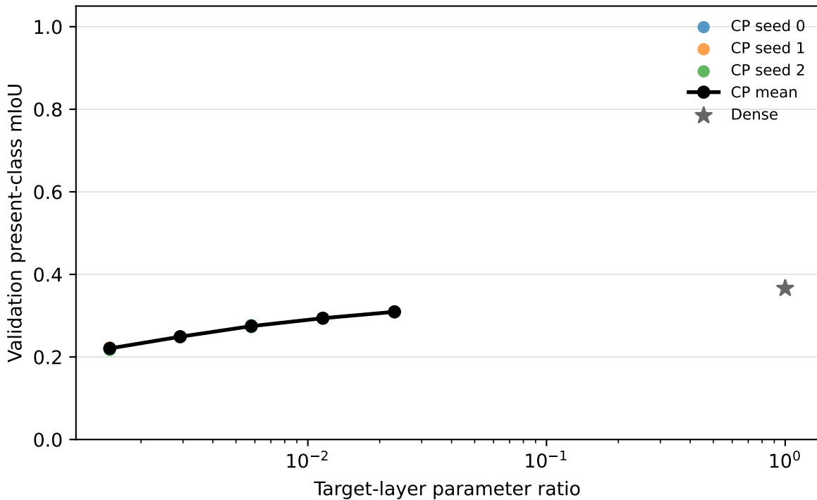
Zero-shot segmentation at the final structural protocol
