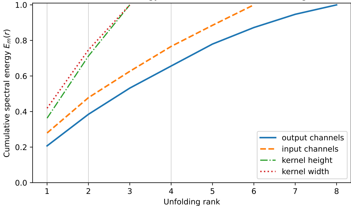
Cumulative energy of convolution-tensor unfoldings
