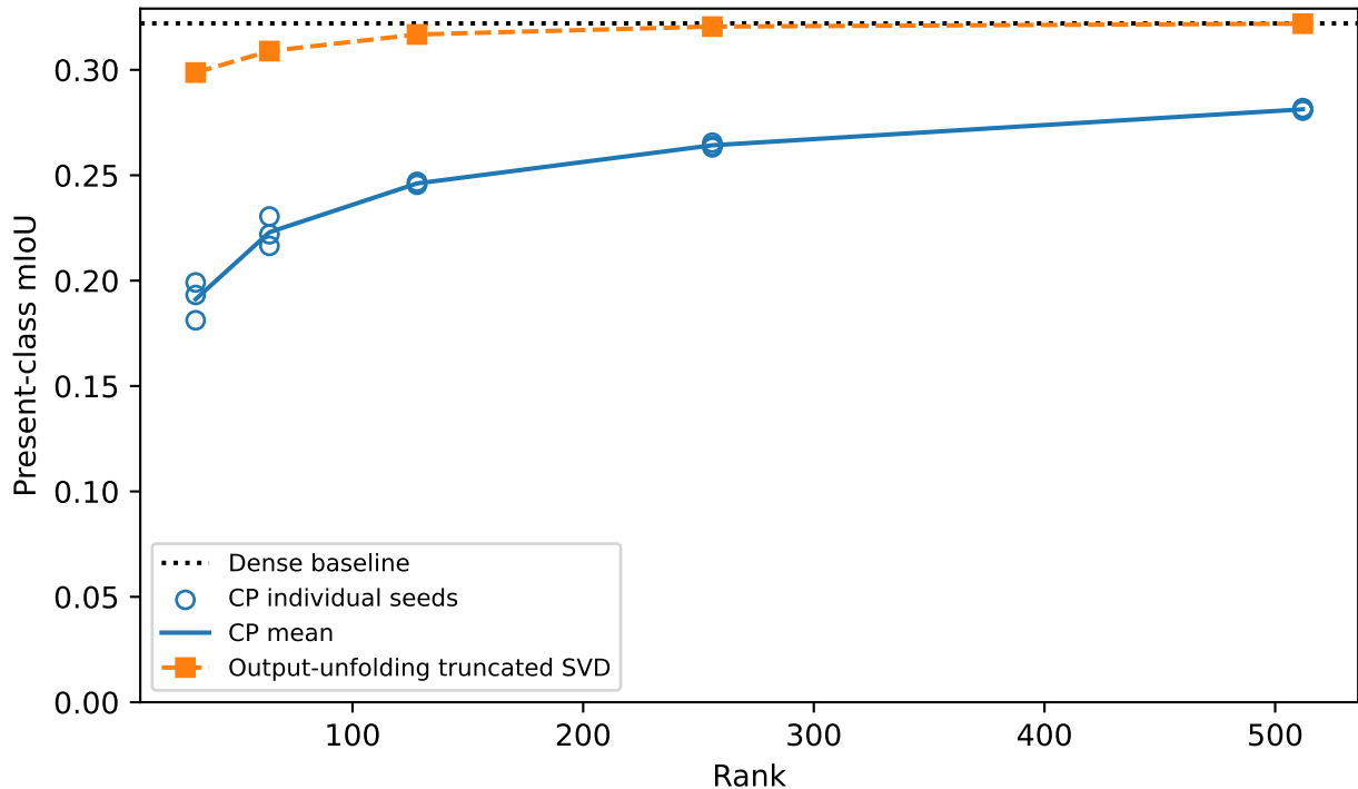
Zero-shot present-class mIoU on the CamVid test split
