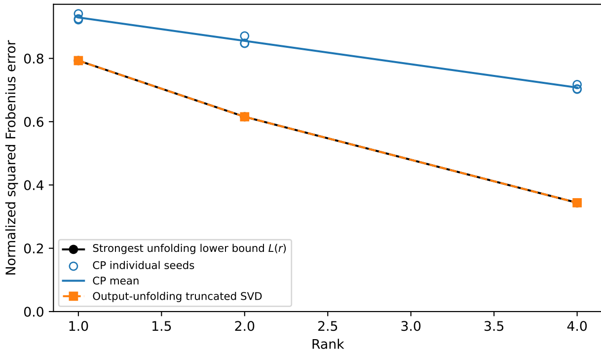
Unfolding lower bound and actual weight reconstruction error
