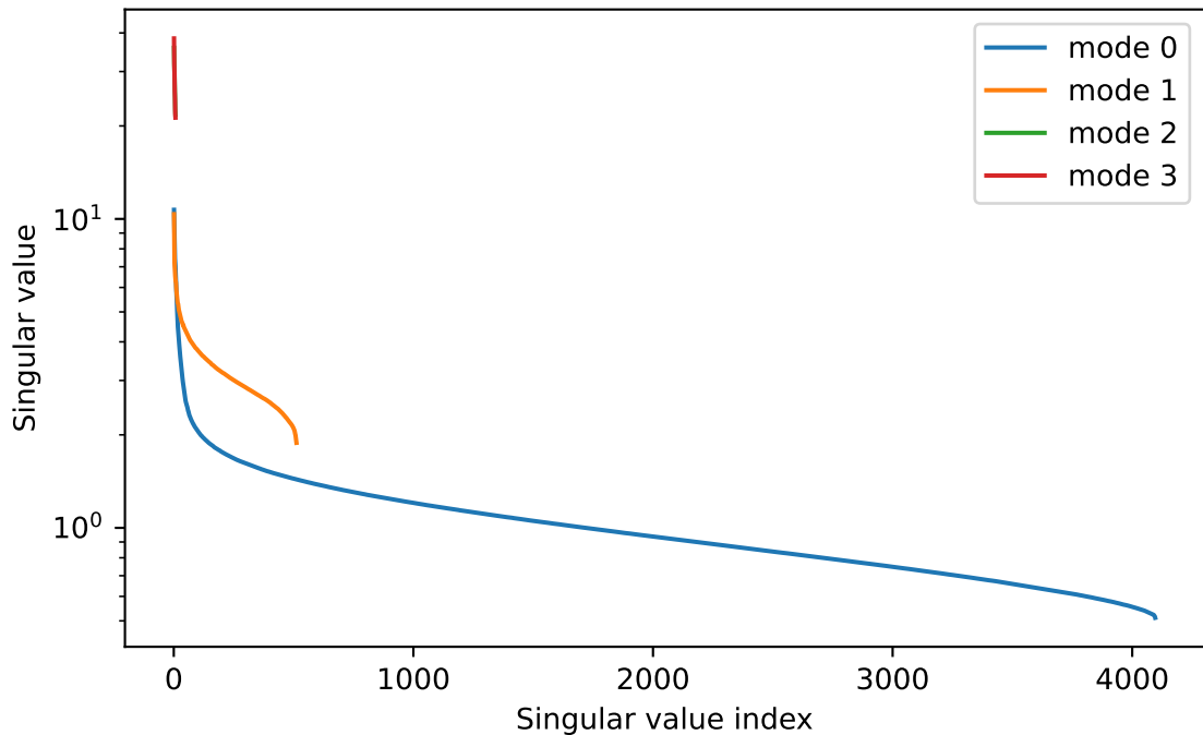
Singular value decay by unfolding mode
