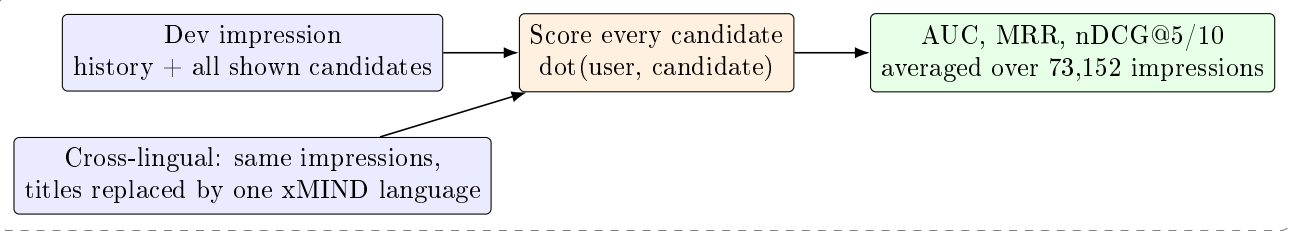
evaluation on MINDsmall dev
