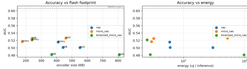
Fig. 2. Accuracy vs. encoder flash (left) and vs. the Horowitz energy estimate (right, log axis), per arm and precision; dashed line: 27 MB NRMS baseline (0.607).
