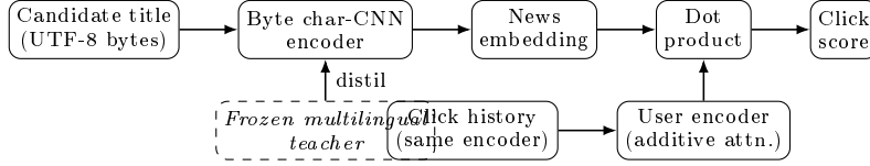
Fig. 1. The recommender: a byte char-CNN (distilled from a frozen multilingual teacher) embeds candidate and history titles; an additive-attention encoder pools the history and a dot product scores the candidate. Only the char-CNN is searched and quantised.
