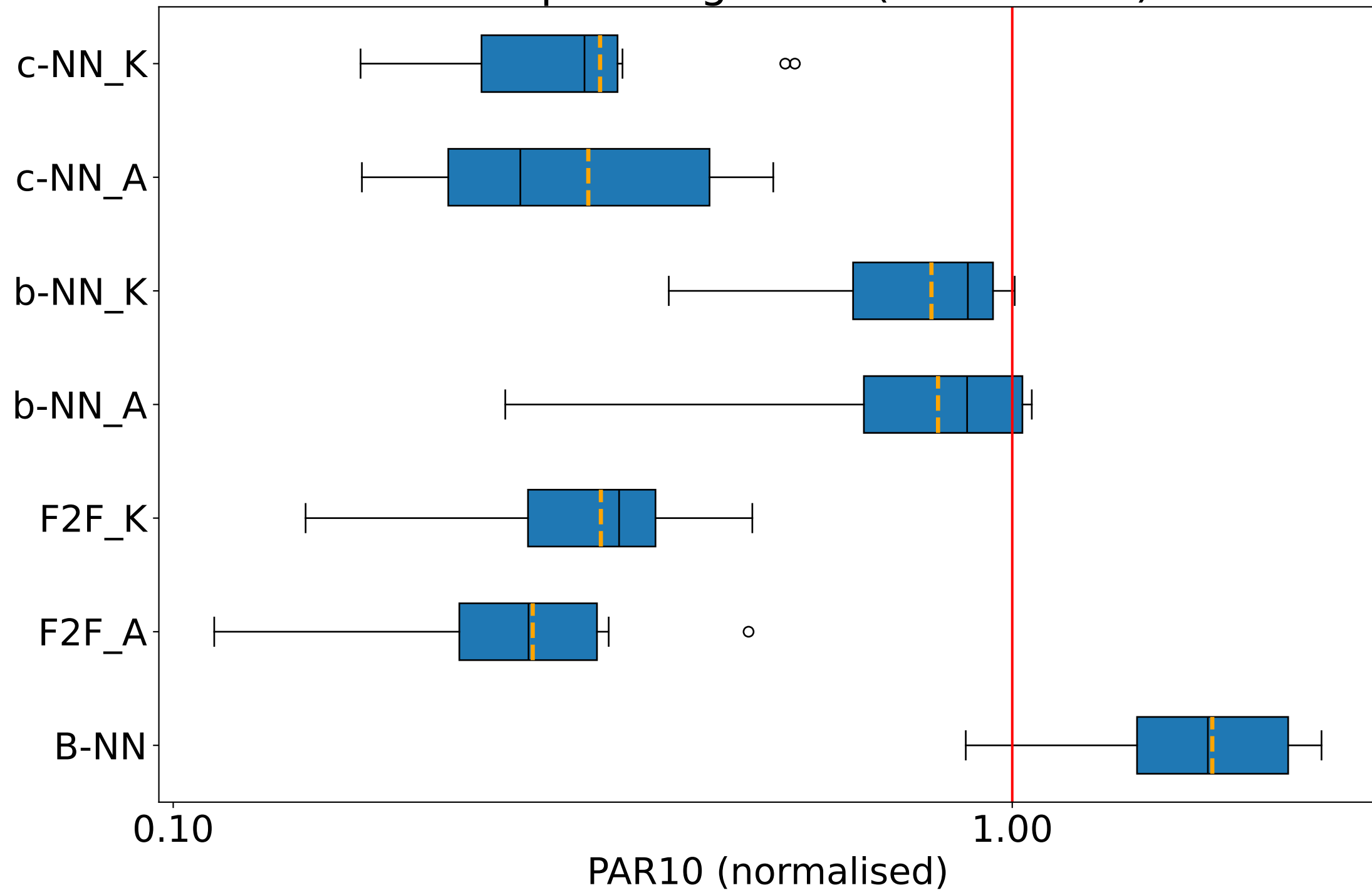
Car sequencing - Test (normalised)
