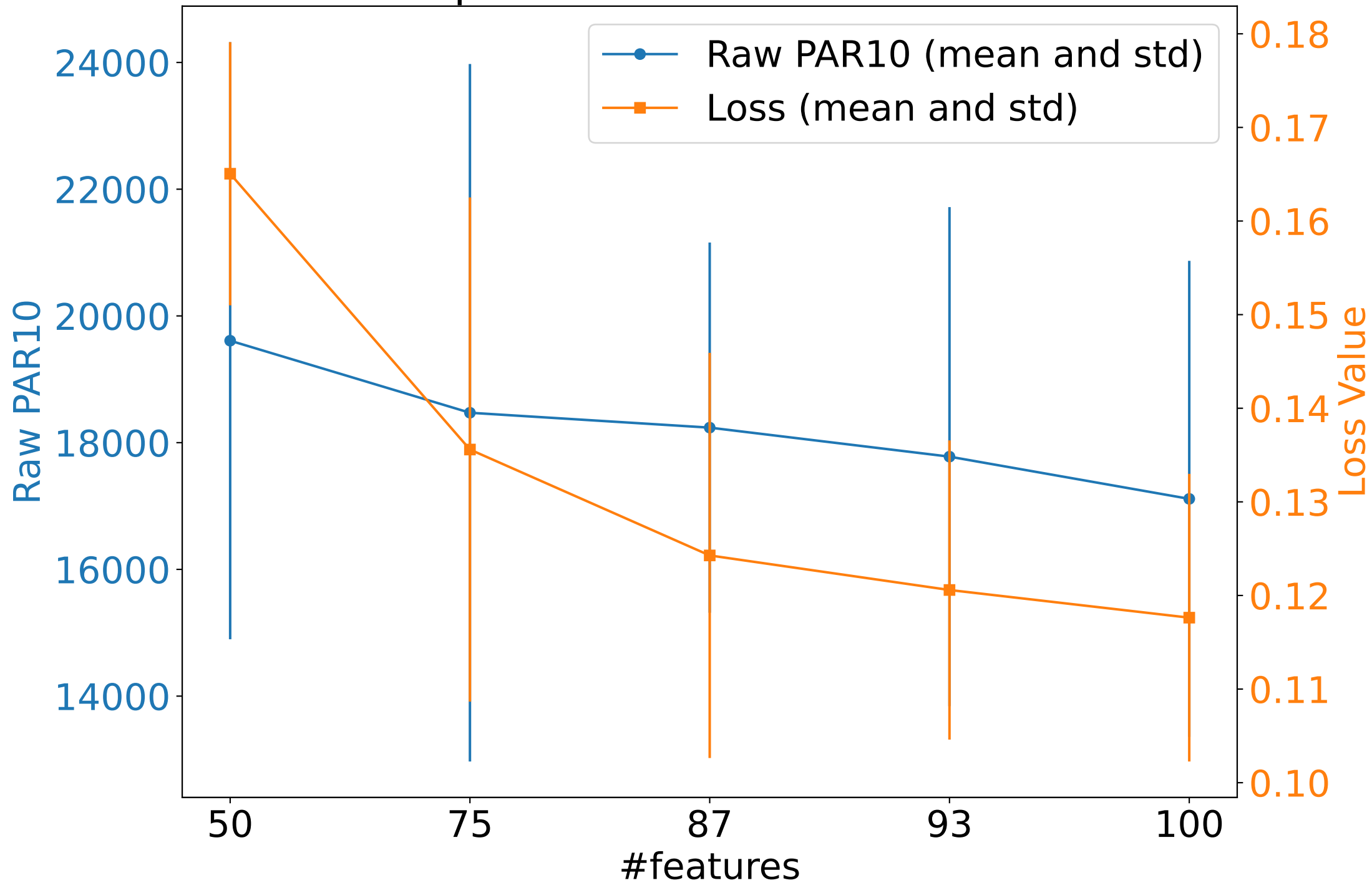
Score per #features - Social Golfers
