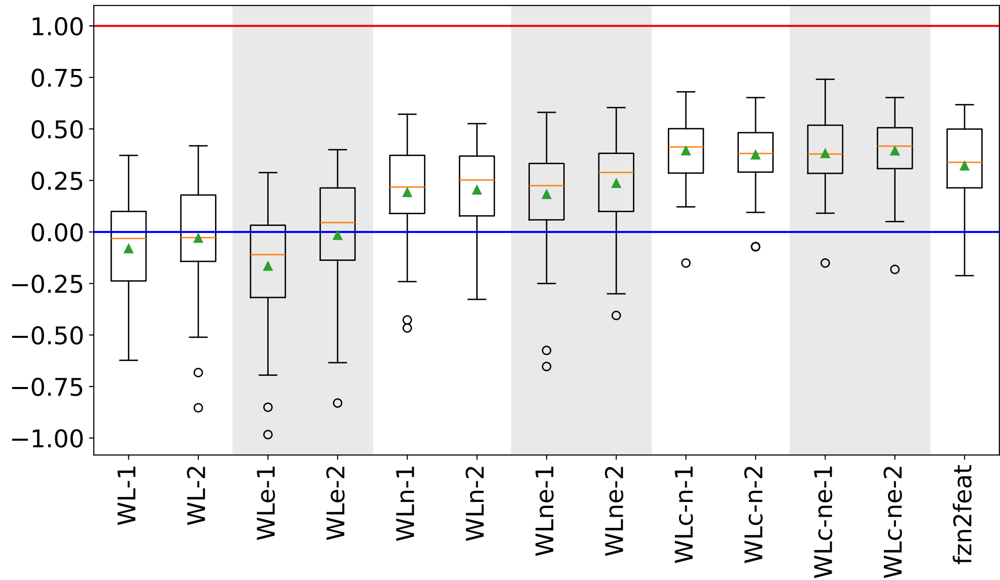
MLP Borda Count Scores
