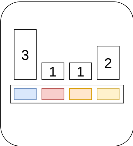
Feature Extraction
