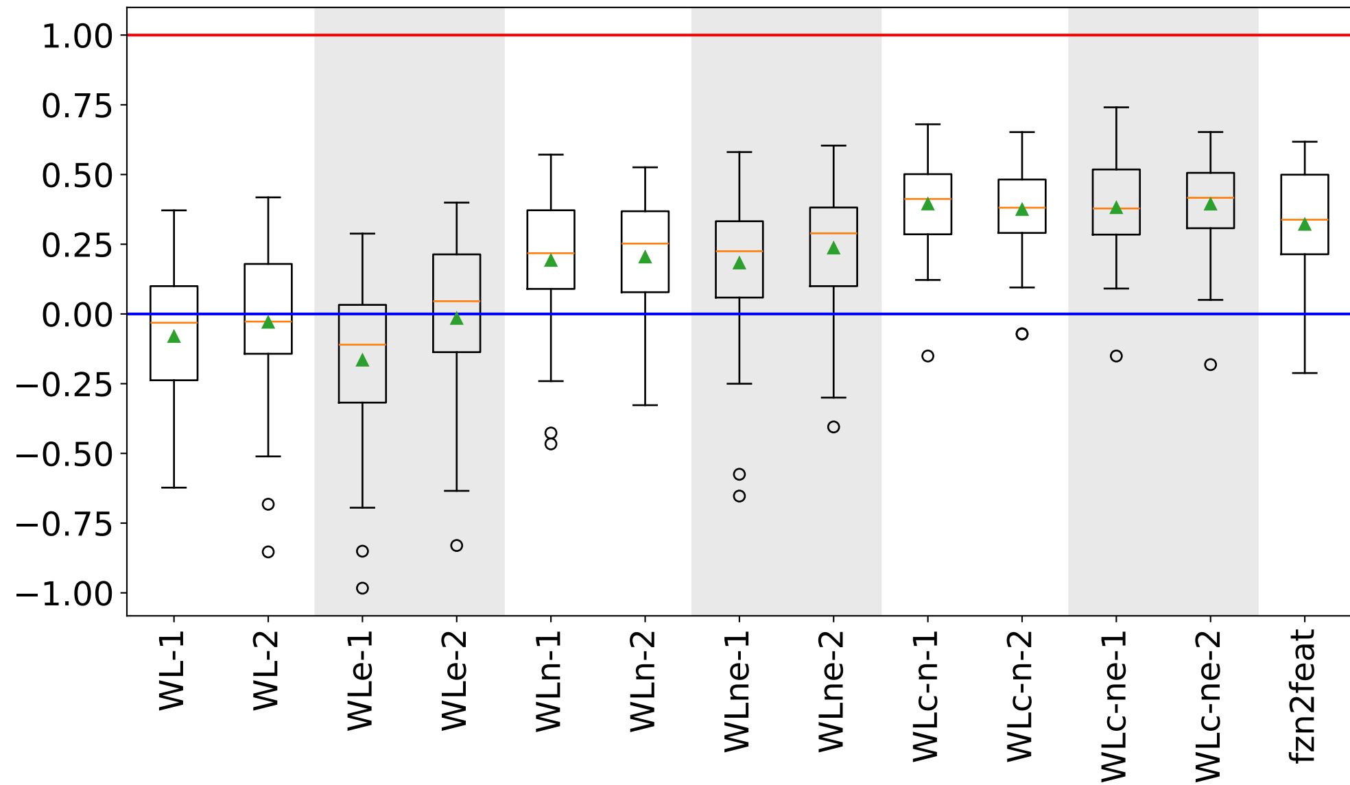
Random Forest Borda Count Scores
