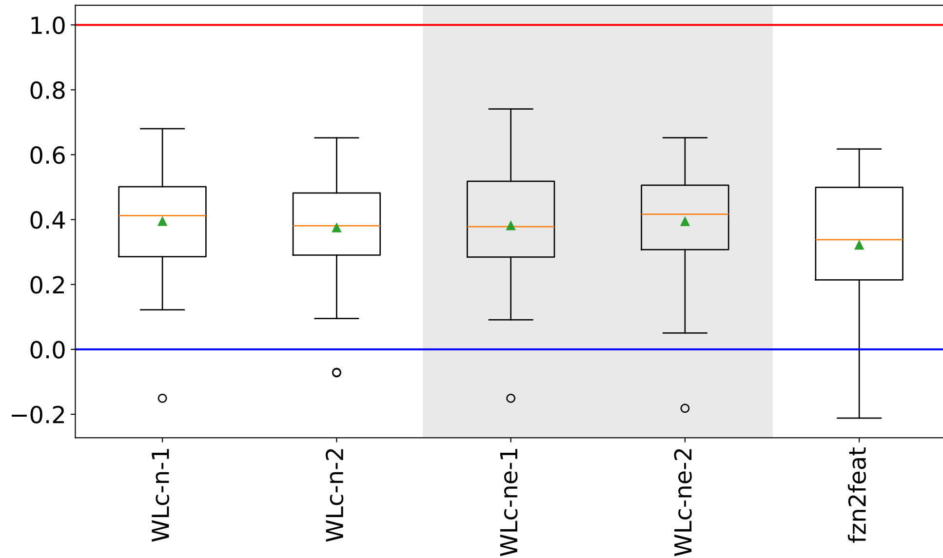
Random Forest Borda Count Scores
