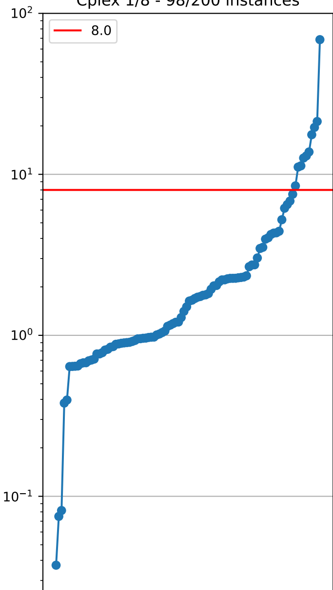
Cplex 1/8 - 98/200 instances
