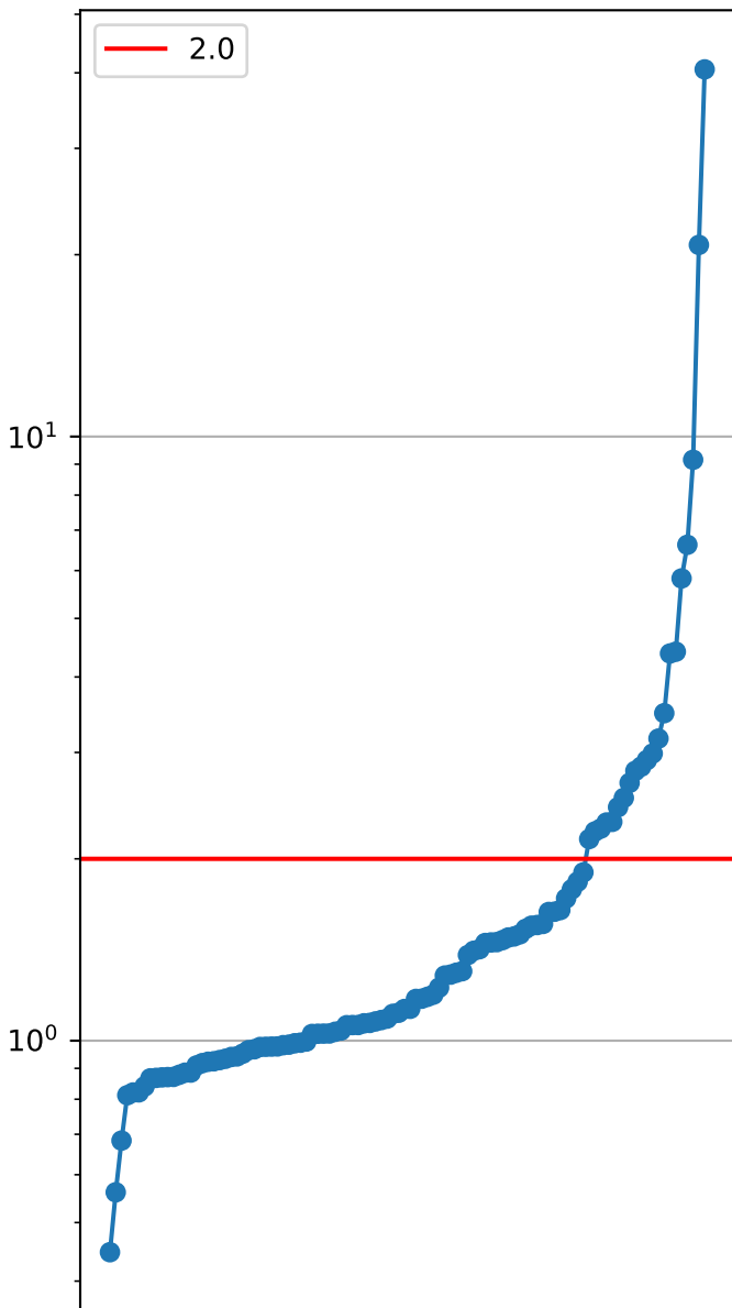
Cplex 2/4 - 104/200 instances
