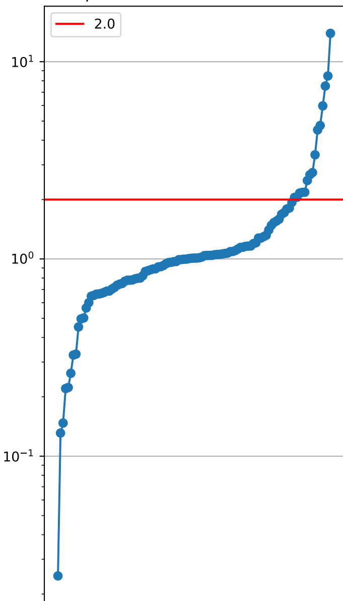
Cplex 4/8 - 107/200 instances
