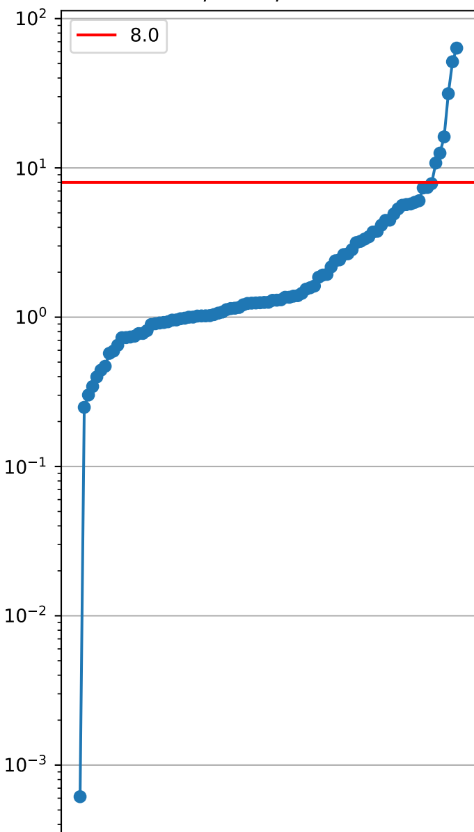
Gecode 1/8 - 91/200 instances
