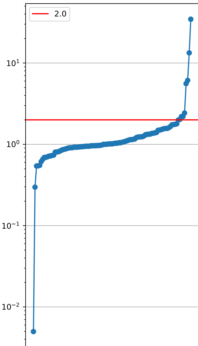
Gecode 4/8 - 102/200 instances
