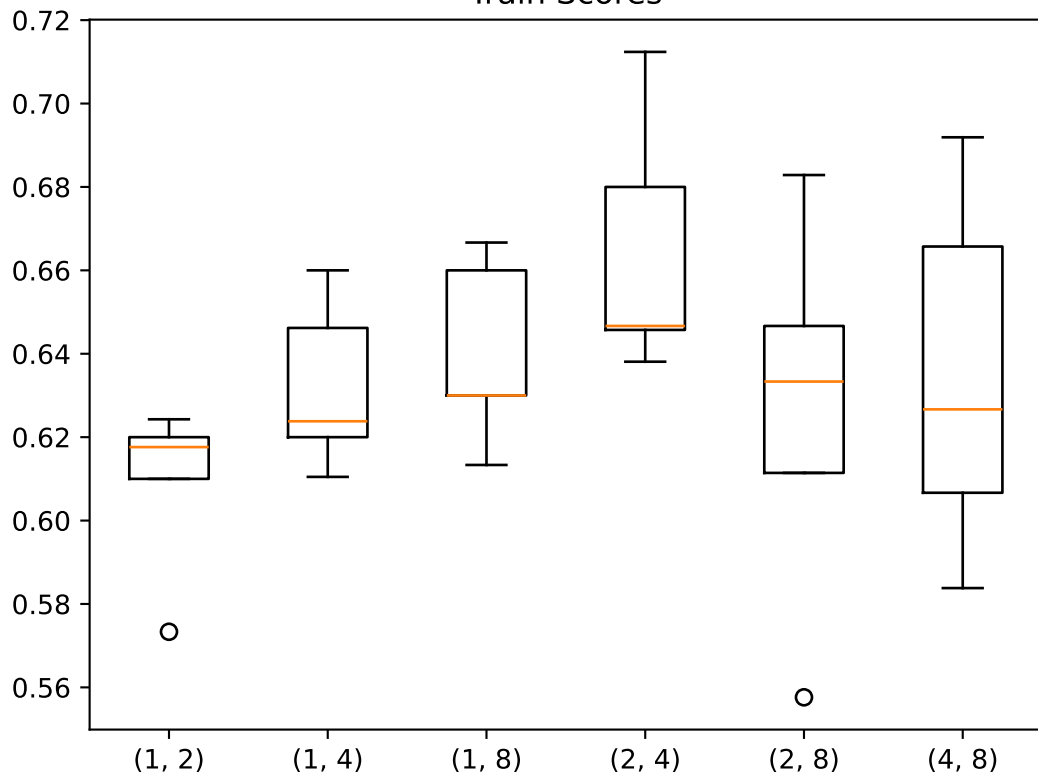
Train Scores
