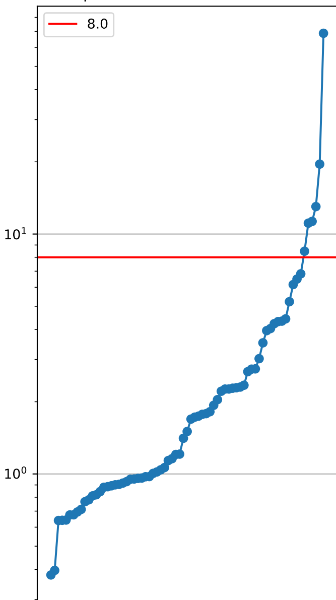
Cplex 1/8 - 73/200 instances
