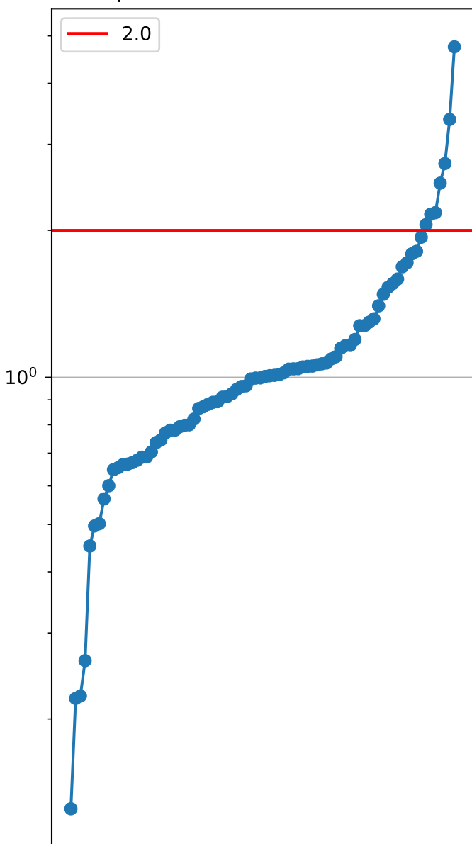
Cplex 4/8 - 82/200 instances
