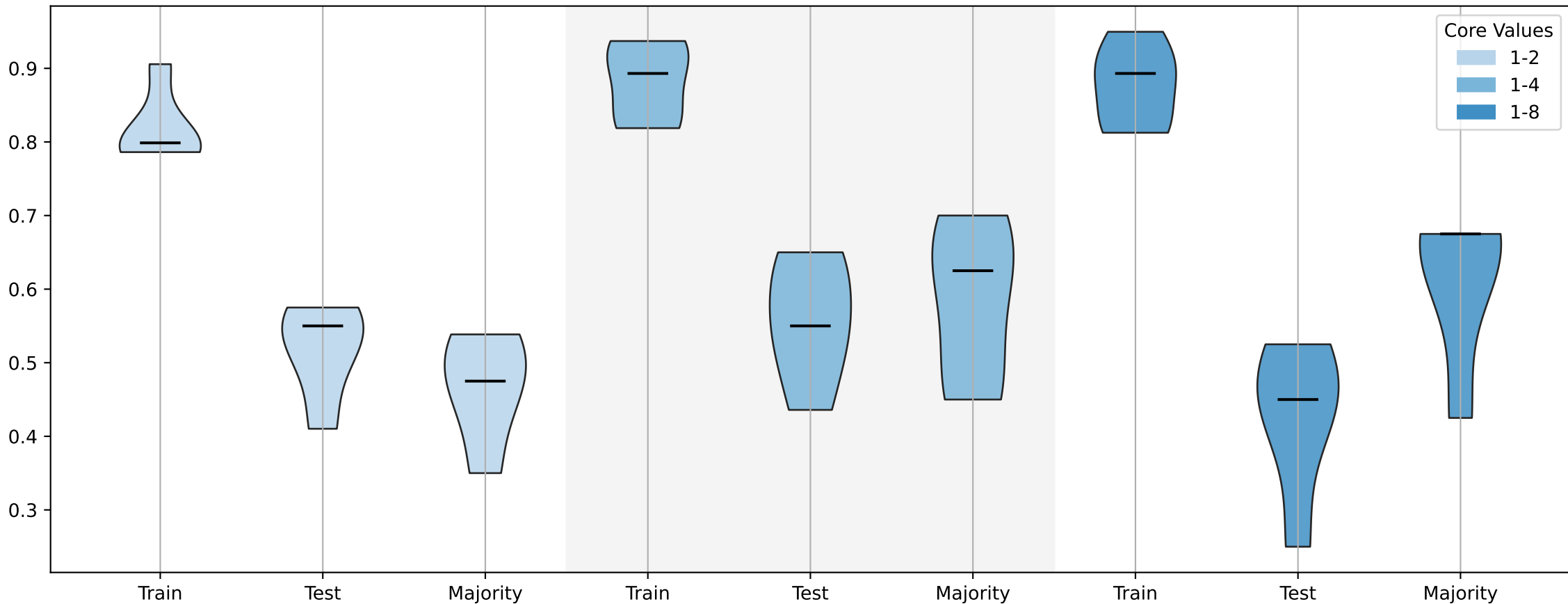
Cplex Scores (Problem-unaware)
