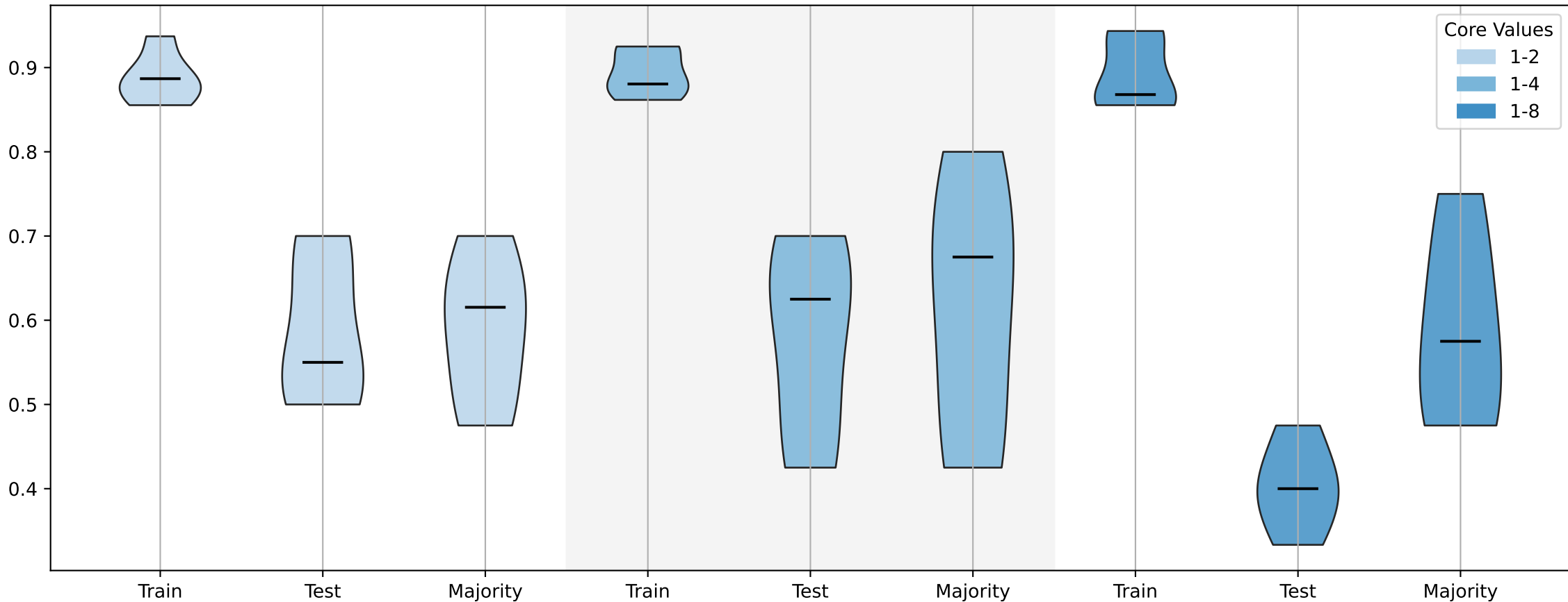
Gecode Scores (Problem-unaware)
