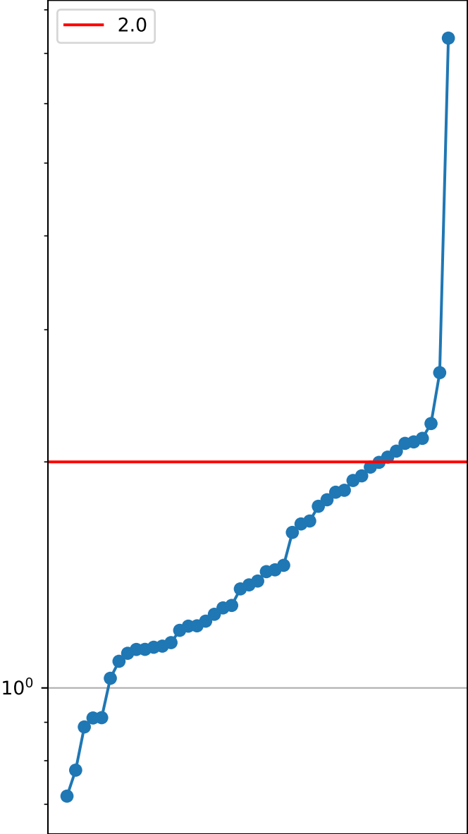
Gecode 1/2 - 45/200 instances
